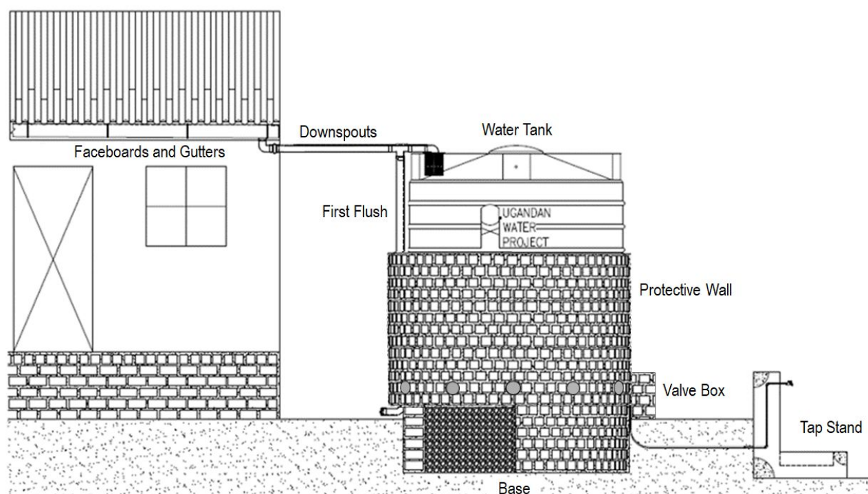
Figure 1: Schematic diagram of a UWP rainwater catchment system
